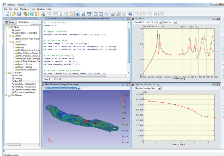
Topometry optimization to reduce the maximum FRF-level.
