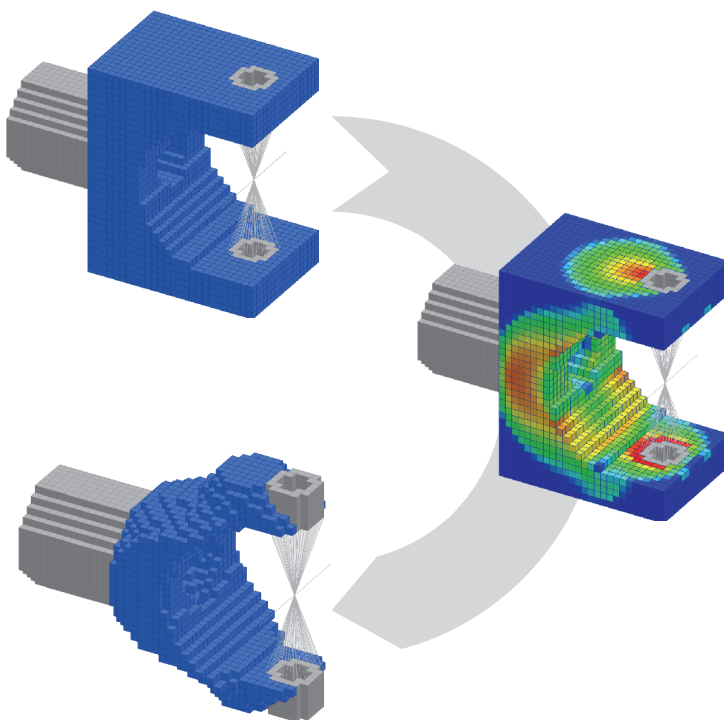
Topology optimization of a joint bracket.
