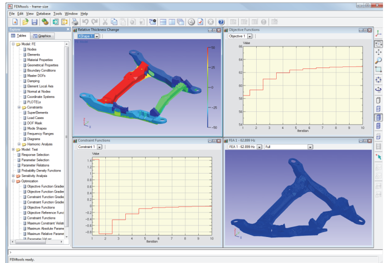
Size optimization of engine frame plate thickness.
