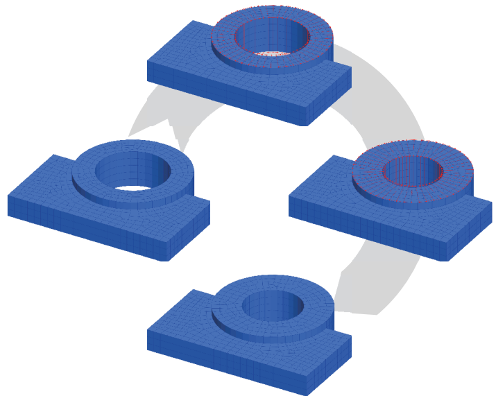
Modifying the inner diameter of a ring using mesh morphing.
